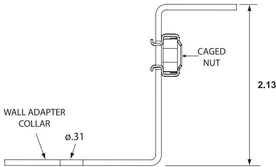
Figure 1 Section A-A
